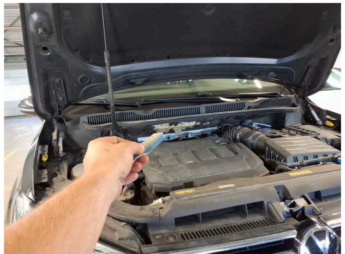
Damage 2: Bonnet: Insulation lining (Stirnwand matte) - Broken / torn - Replace
