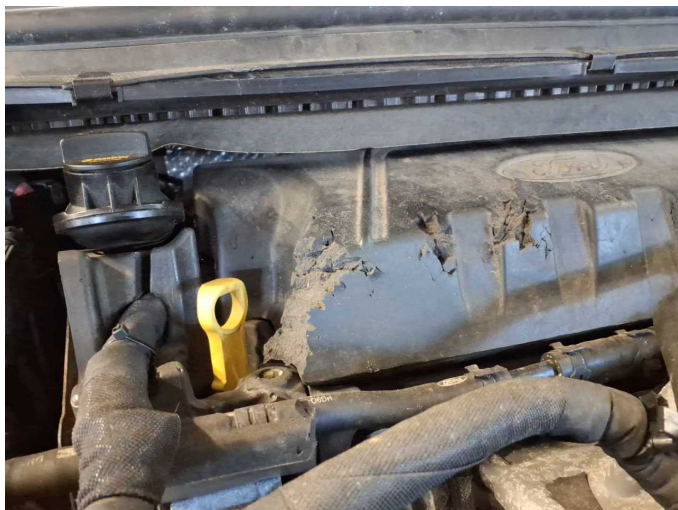
Damage 6: Engine: Engine cover - top / cover (Marderschaden) - Broken / torn - Replace
