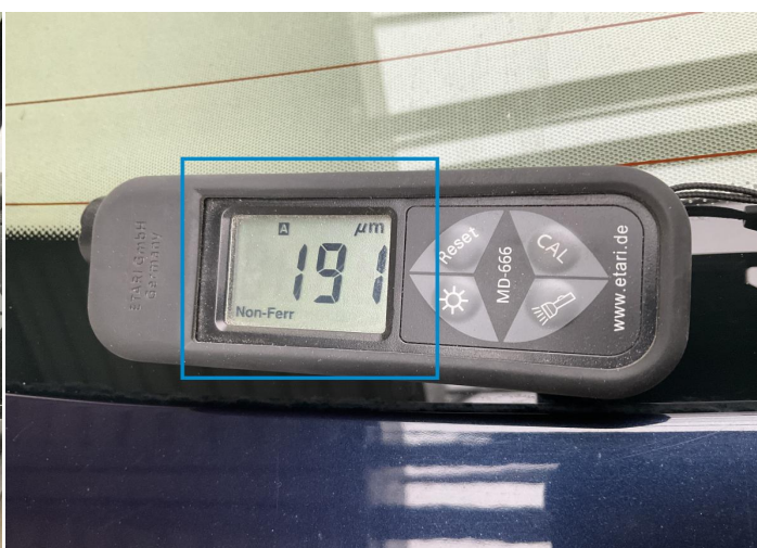
6. Tailgate Paint / Poor Previous Repair -
