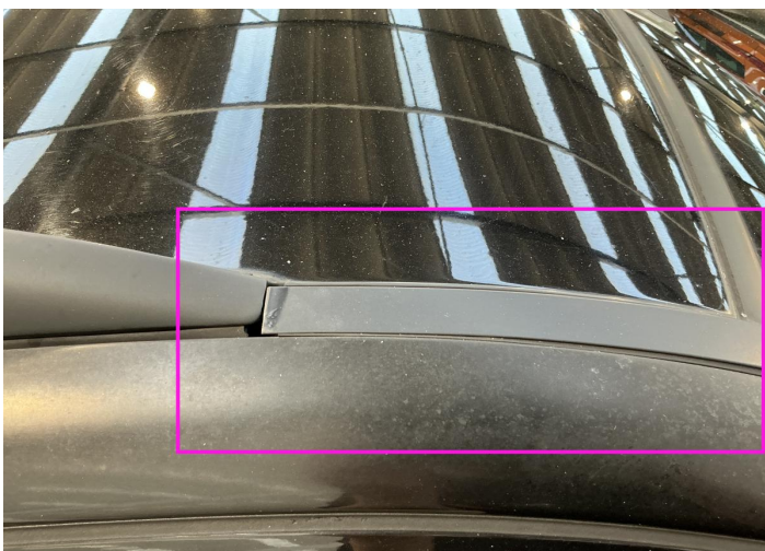
18. Roof Molding / Right Out of Bodywork / Breakage -
