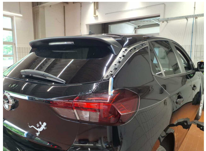
Damage 7: Side panel - rear right side: Protection strip (Hinten rechts) - Broken / torn - Replace
