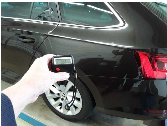
Side panel - rear left side: 581 µm
