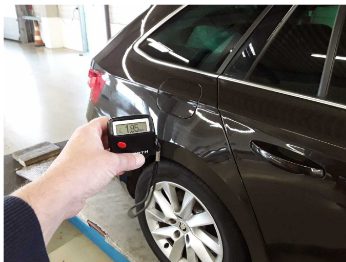
Side panel - rear right side: 1,950 µm
